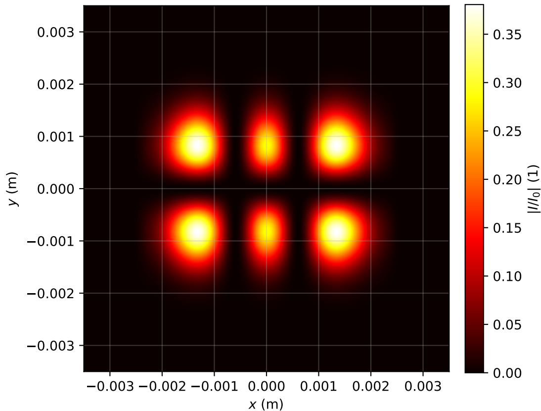
Intensity profile I(x, y, z = 2.707)/I_0 , P_{in}=0.5P_{cr} , artificial time
